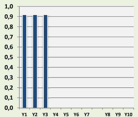
CDD Framework
